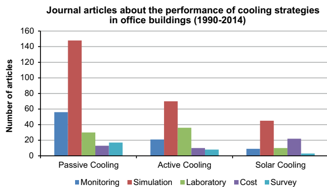
Fig. 8. Cooling articles considering diverse research methods.
