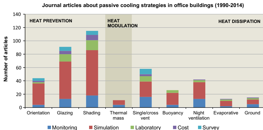
Fig. 9. Passive cooling strategies in articles considering diverse research methods.
